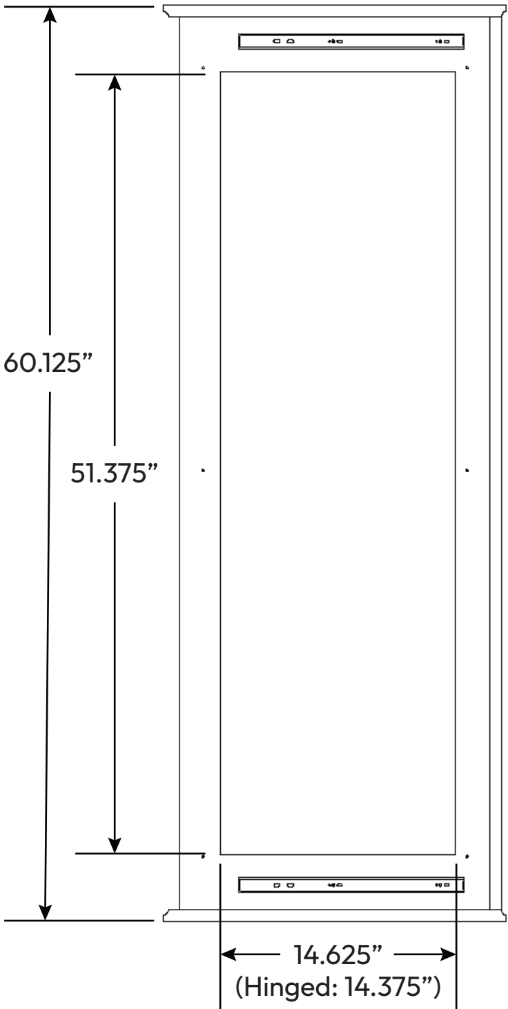
Frame Only
